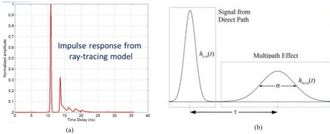
FIGURE 3. (a) Impulse response from ray-tracing model; (b) Multipath Effect
