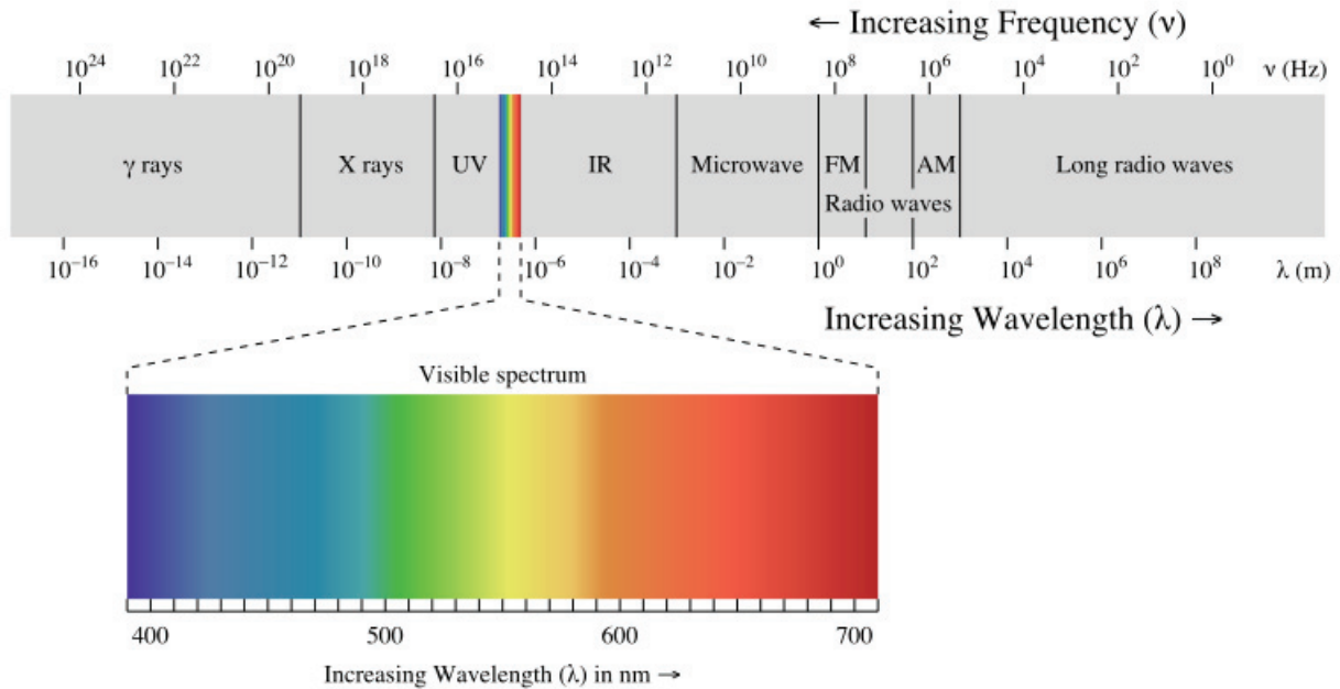
FIGURE 1. The human eye can sense the electromagnetic signals between the frequency range of 430 THz and 790 THz
