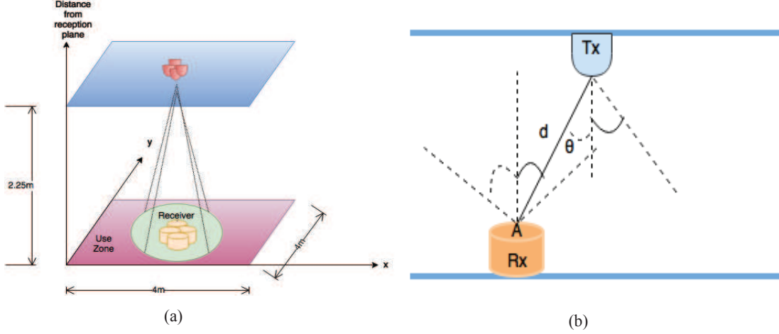
FIGURE 4. (a) MIMO system in a typical room scenario; (b) System model with simulation parameters
